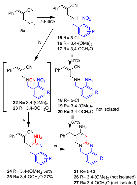
Scheme 4. Reagents and conditions- i) a) Substituted 2-nitrobenzaldehyde, CH 2 Cl 2 , rt, 3h. b) NaBH(OAc) 3 , C 6 H 6 , 0°C-rt, 8h. ii) In-HCl, THF: H 2 O (1:1, v/v), rt, 1.5 h. iii) a) CNBr, MeOH, rt, 30 min. b) NaOMe, MeOH, rt, 1 h. iv) CNBr, THF, rt, 30 min. v) In-HCl, H 2 O, rt, 1.5 h
