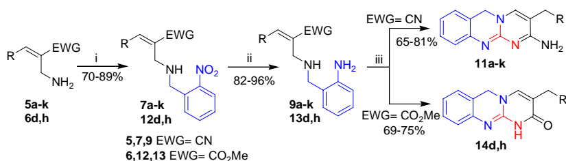
Scheme 3. Reagents and conditions- i) a) 2-Nitrobenzaldehyde, \text{CH}_2\text{Cl}_2 , rt, 3h. b) \text{NaB}(\text{OAc})_3 , \text{C}_6\text{H}_6 , 0^\circ\text{C} -rt, 8h. ii) \text{In-HCl} , THF: \text{H}_2\text{O} (1:1, v/v), rt, 1.5 h. iii) a) \text{CNBr} , MeOH, rt, 30 min. b) \text{NaOMe} , MeOH, reflux, 4 h for 9 (one-pot) and \text{NaOMe} , MeOH, rt, 1.5 h for 13 (one-pot).
