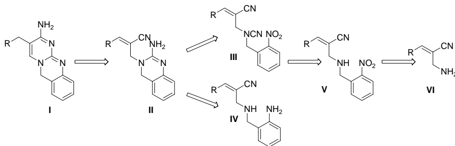
Figure 1. Retrosynthetic analysis for the preparation of pyrimido[2,1-b]quinazoline from the primary allyl amine afforded from the Baylis-Hillman adduct.
