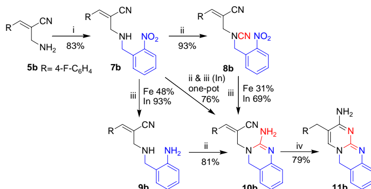
Scheme 2. Reagents and conditions- i) a) 2-Nitrobenzaldehyde, \text{CH}_2\text{Cl}_2 , rt, 3 h. b) \text{NaBH}(\text{OAc})_3 , \text{C}_6\text{H}_6 , 0^\circ\text{C} -rt, 8 h. ii) \text{CNBr} , THF or MeOH, rt, 30 min. iii) \text{Fe-AcOH} , 90^\circ\text{C} , 1 h or \text{In-HCl} , THF: \text{H}_2\text{O} (1:1, v/v), rt, 1.5 h. iv) \text{NaOMe} , MeOH, reflux, 4 h.
