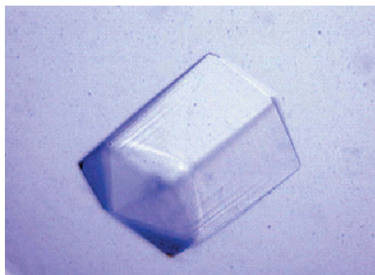
Figure 1 Crystal of B. anthracis nucleoside diphosphate kinase.
