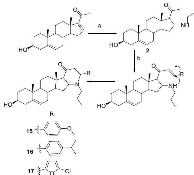
Scheme 2: Synthesis of Aza derivatives of 16-dehydropregnenolone. Reagents and conditions: (a) propyl amine, 45° C, 4 h. (b) RCHO, EtOH, KOH, rt, 24 h.
