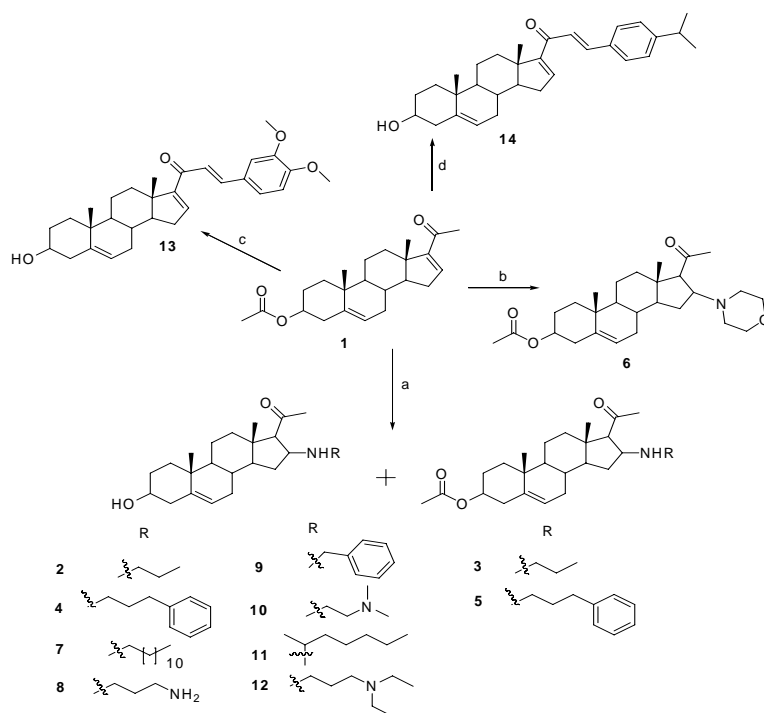
Scheme 1. Synthesis of different amine derivatives of acetylated 16-dehydropregnenolone. Reagents and conditions: (a) RNH 2 , 45° C, 4h. (b) morpholine, 45° C, 4h. (c) 3,4-dimethoxy benzaldehyde, EtOH, KOH, rt, 24 h. (d) 4-isopropyl benzaldehyde, EtOH, KOH, rt, 24h
