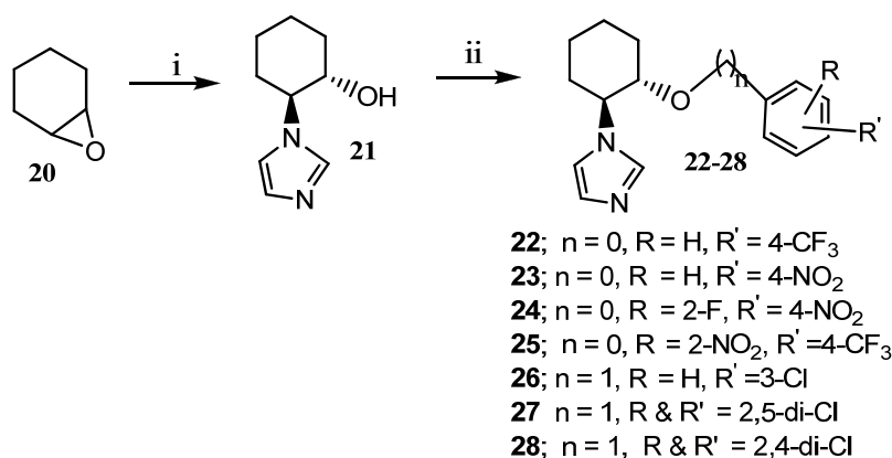
Scheme 3. Reagents and conditions: (i) Imidazole, abs. ethanol, 90°C, 12h; (ii) NaH (60% Oil), substituted aryl or benzyl halide, DMF, 0°C-rt, 4-5h.
