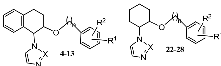
Figure 1. Aryloxy tetrahydronaphthyl and cyclohexyl azoles
