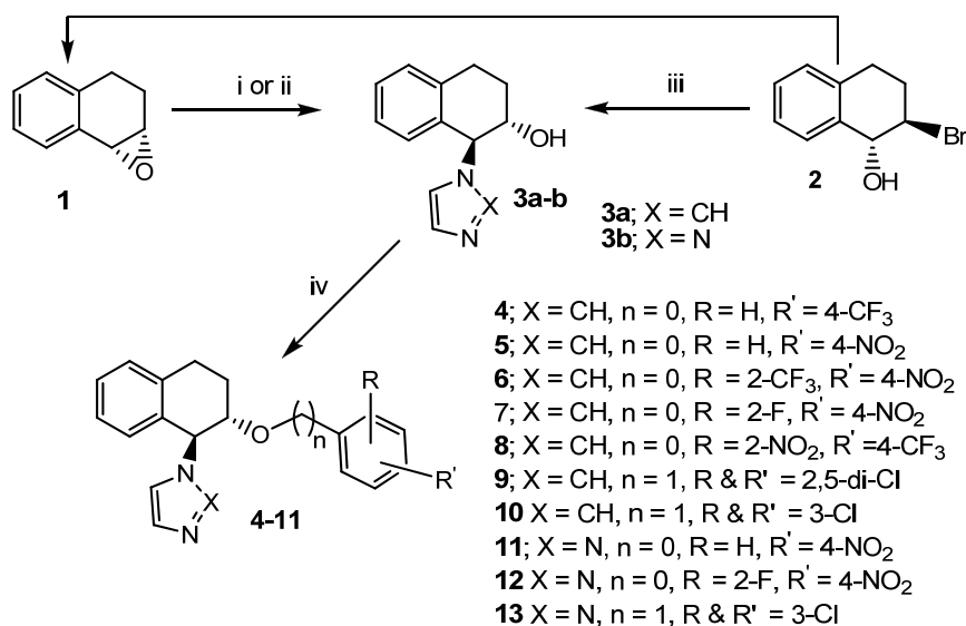
Scheme 1. Reagents and conditions: (i) Imidazole / abs. ethanol. (ii) 1,2,3-triazole / (But) 4 N + I - . (iii) Imidazole / acetonitrile. (iv) NaH (60 % Oil), substituted aryl or halo benzene / DMF.
