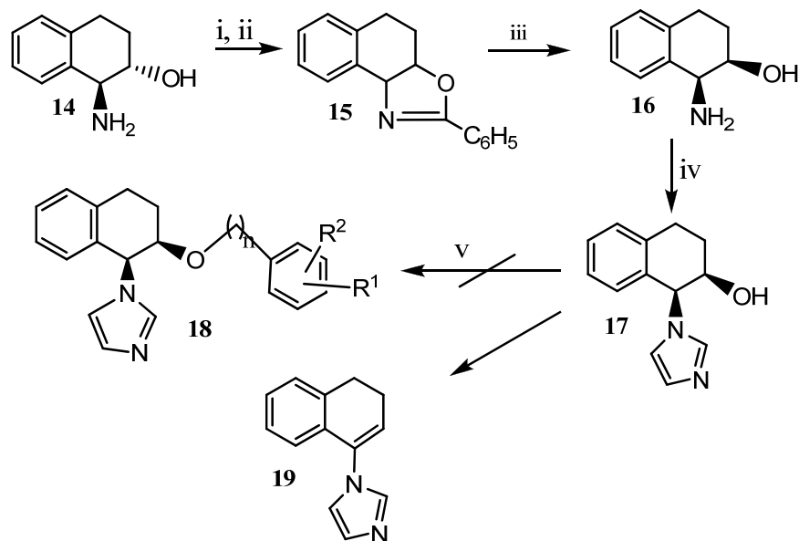
Scheme 2. Reagents and conditions: (i) PhCOCl, KOH, H 2 O, rt, 3h; (ii) SOCl 2 , CH 2 Cl 2 , rt, 7h; (iii) 6N.H 2 SO 4 , reflux, 11h; (iv) glyoxal, NH 4 OAc, HCHO, methanol, 80°C, 8h; (v) NaH (60% Oil), substituted aryl or benzyl halide, DMF, 0°C-rt, 4-5h.
