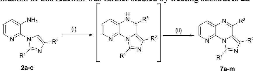
Scheme 2. Reagents and conditions: (i) R 3 CHO, 1% TFA in toluene, 120 °C. (ii) DDQ, 10 min
