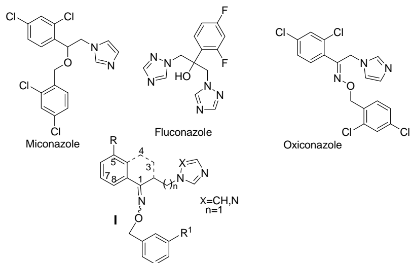
Figure 1. Representative azole drugs
