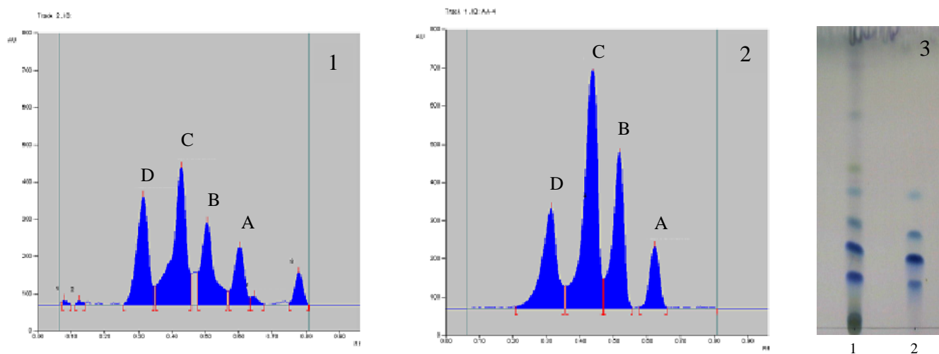
Fig. 2 The representative HPTLC chromatograms (1, 2) and Photo-documentation (3) after derivatization of A. nepalensis leaf extract (1) and mixture of standards (2).
