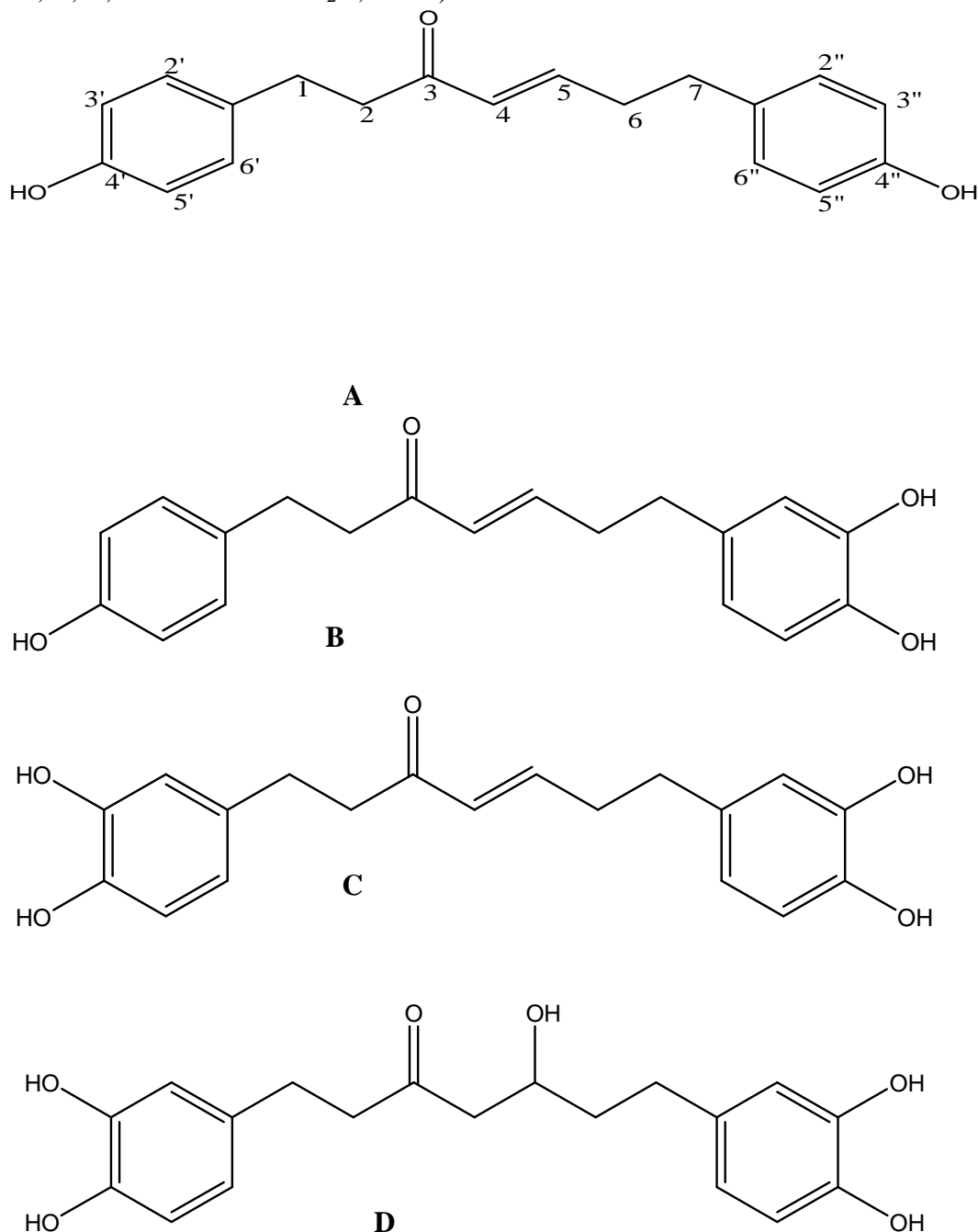
Fig. 1 Chemical Structures of Compounds A , B , C and D .
