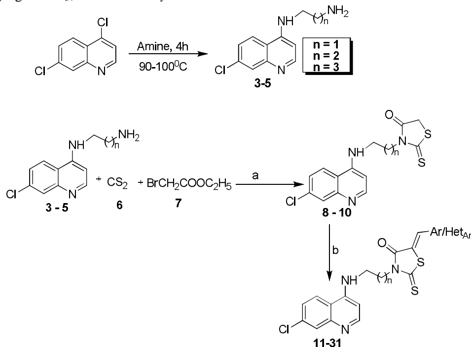
Scheme 1. Synthesis of 4-aminoquinoline-rhodanine hybrids.
