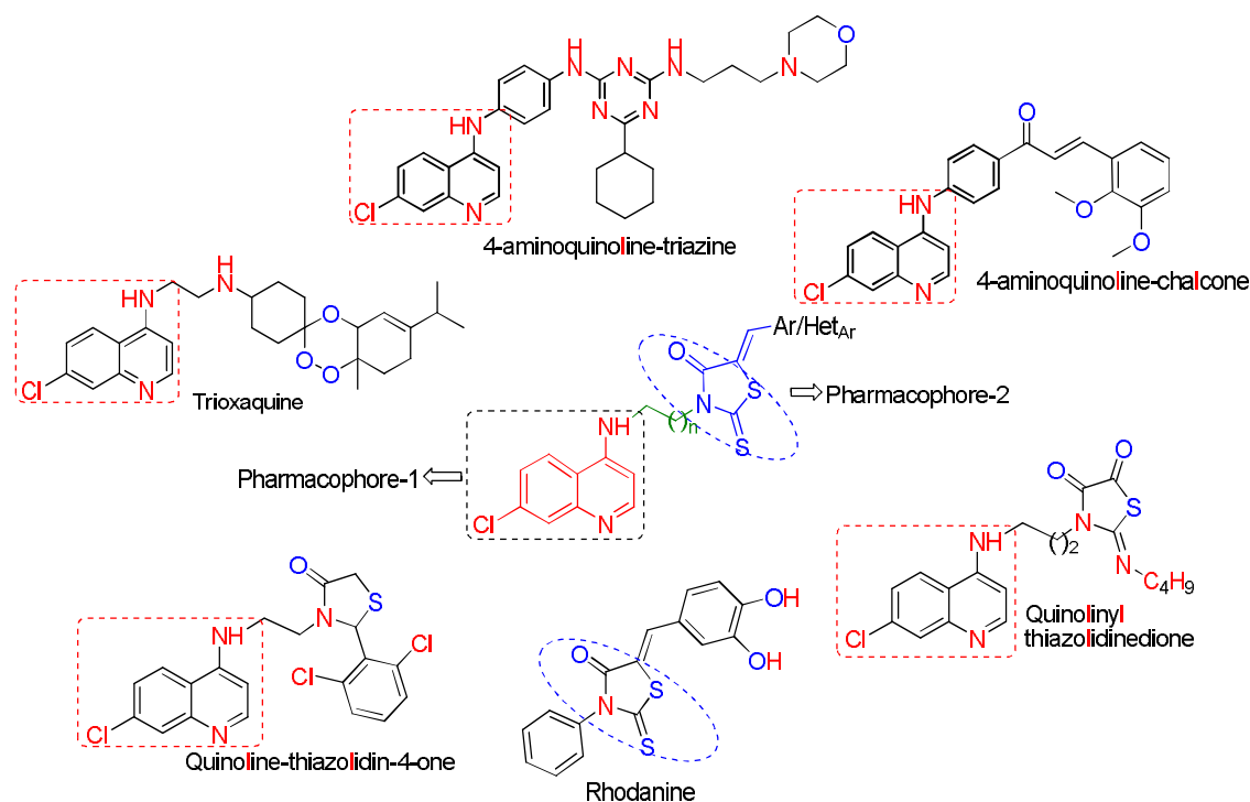
Figure 1. Designing of 4-aminoquinoline-rhodanine hybrid based on 4-aminoquinoline and rhodanine scaffolds showing antimalarial and antitubercular activity
